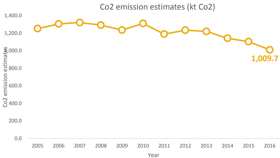
Figure 1: Annual CO 2 emission estimates (kt CO 2 ) for DCSDC, 2005 to 2016
